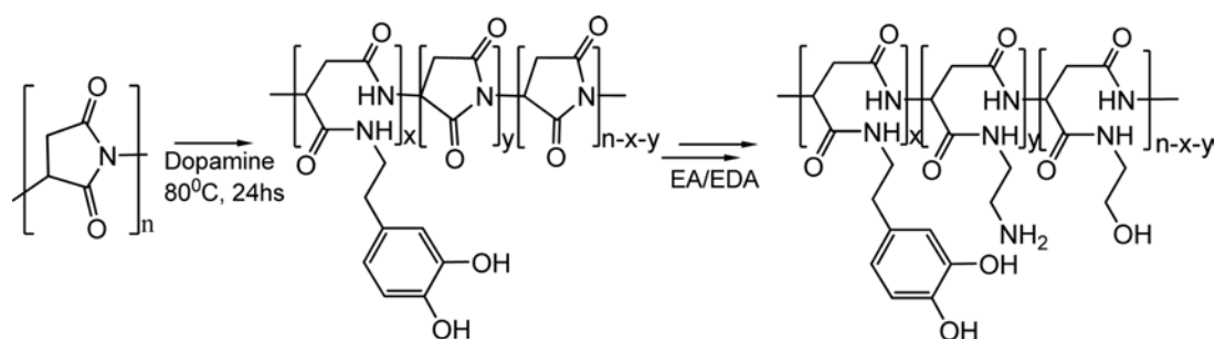
Scheme 2. Synthesis of dopamine-modified polyaspartamide copolymer.
