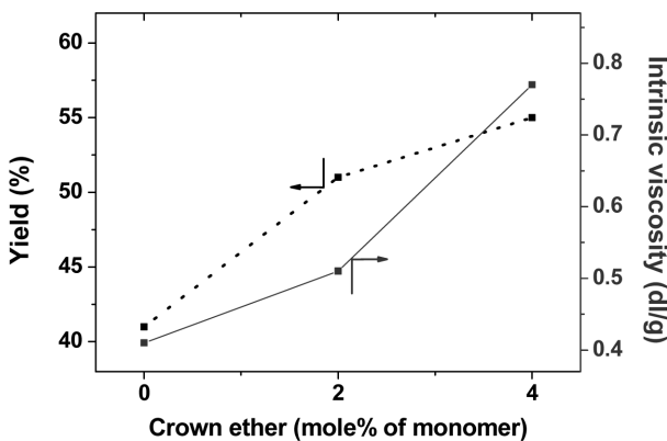
Figure 5. Effect of the amount of crown ether on the intrinsic viscosity and polymerization yield.
