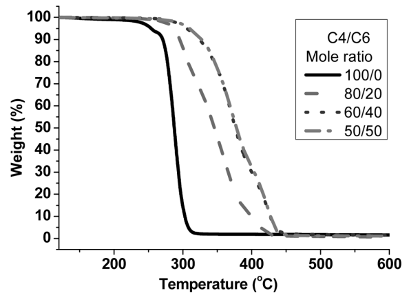
Figure 6. TGA traces of nylon 4/6 copolymer synthesized when crown ether was added.
