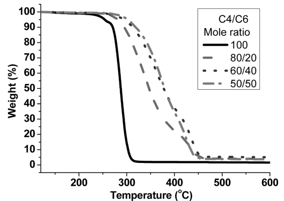
Figure 7. TGA traces of nylon 4/6 copolymer synthesized when TMAC was added.
