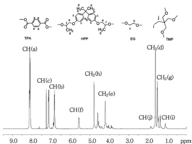
Figure 2. 1 H NMR spectrum of TMP branched copolyester.
