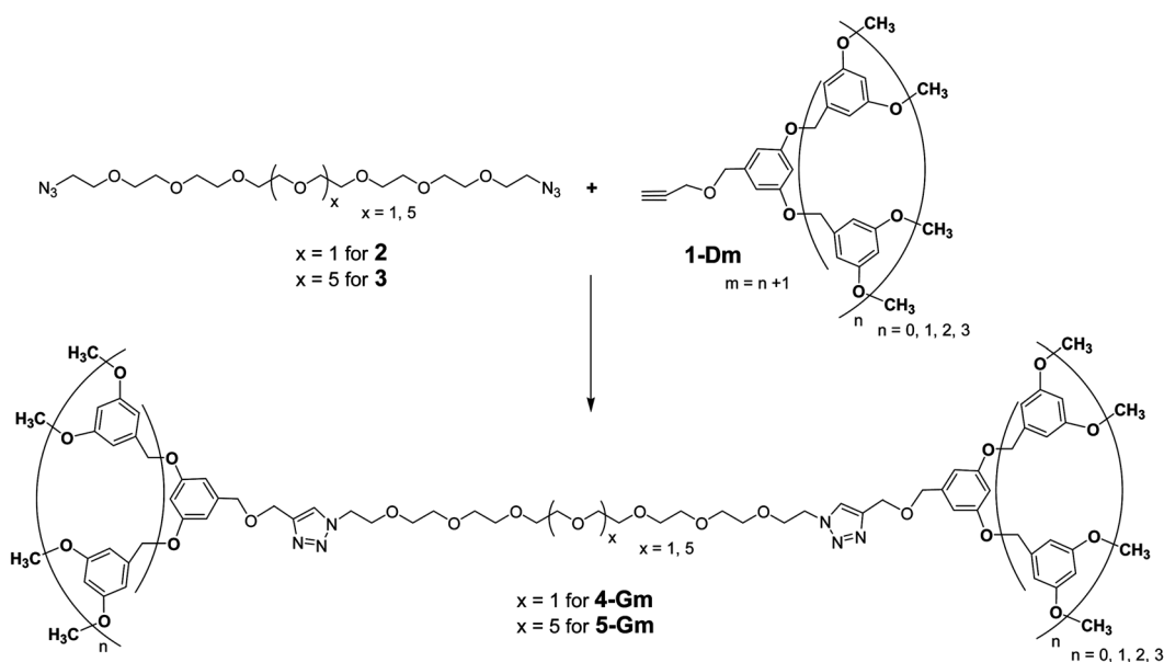
Scheme 1. Synthesis of dendrimers by click reaction between bis-azido-PEG derivatives and alkyne-functionalized dendrons. Reagents and conditions: 10 mol% of CuSO 4 ·5H 2 O/20 mol% of sodium ascorbate, DMF/H 2 O (4:1), 50 °C.
