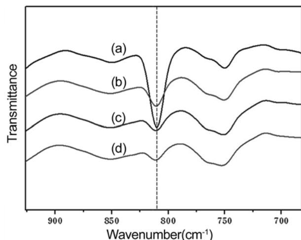
Figure 8. Change in FTIR spectra as a function of irradiation temperature. (a) no irradiation (for comparison); (b) low temperature; (c) room temperature; (d) high temperature.
