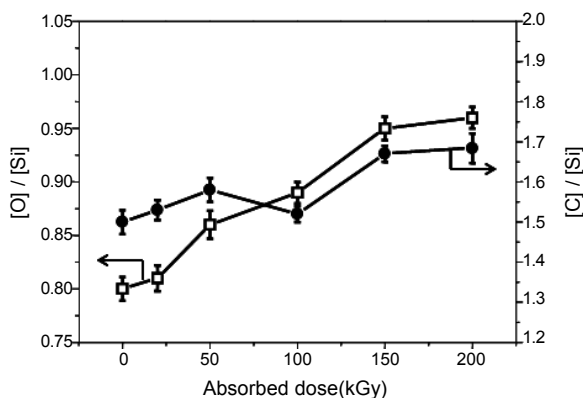
Figure 6. [O]/[Si] and [C]/[Si] atomic concentration ratio of PDMS sheet as a function of absorbed dose as obtained by XPS.
