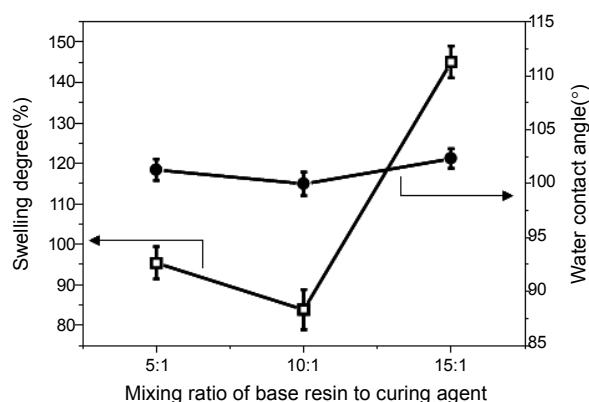
Figure 1. Swelling degree and contact angle of PDMS sheets with various mixing ratios of base resin/curing agent.
