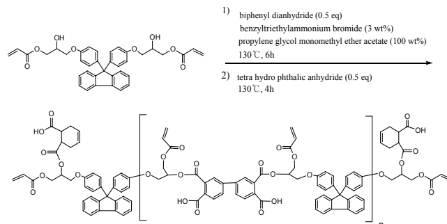
Scheme 3. Condensation polymerization of bisphenol fluorene epoxy acrylate with 4,4'-biphthalic anhydride.
