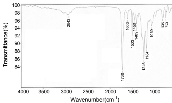
Figure 2. FTIR spectrum of copolymer of bisphenol fluorene epoxy acrylate with bipthalic anhydride.
