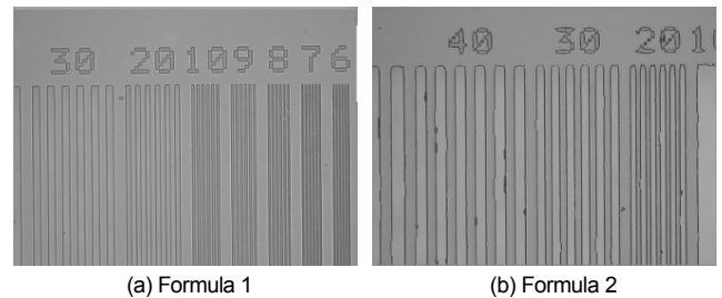
Figure 8. Optical micrographs of BM patterns of (a) formula 1; (b) formula 2.
