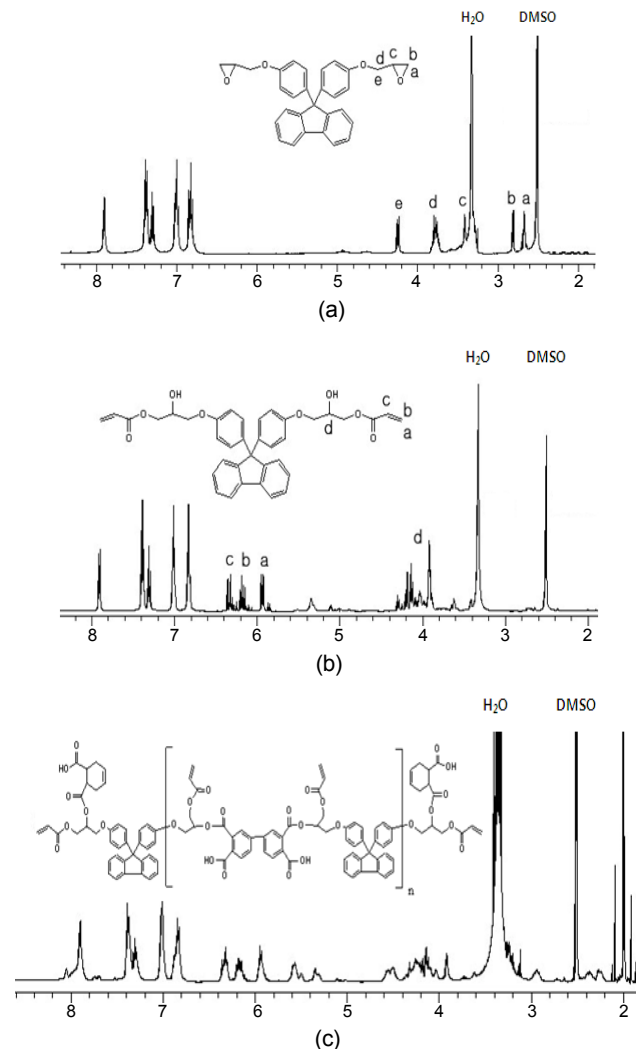
Figure 1. 1 H NMR spectra of (a) epoxy resin containing fluorene moieties; (b) bisphenol fluorene epoxy acrylate; (c) copolymer of bisphenol fluorene epoxy acrylate with biphtalic anhydride.
