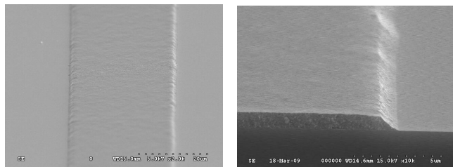
Figure 9. SEM images of CBR BM employing formula 1.
