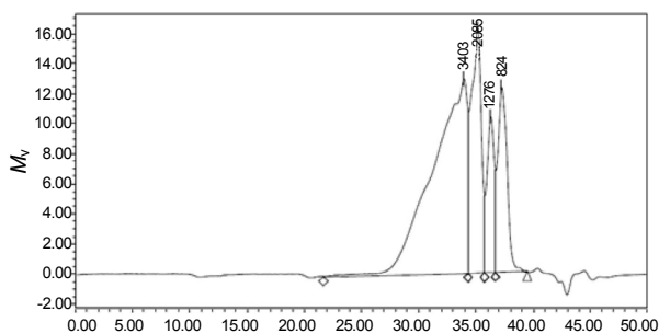
Figure 3. GPC trace of copolymer of bisphenol fluorene epoxy acrylate with bipthalic anhydride.
