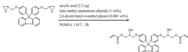
Scheme 2. Synthesis of bisphenol fluorene epoxy acrylate.
