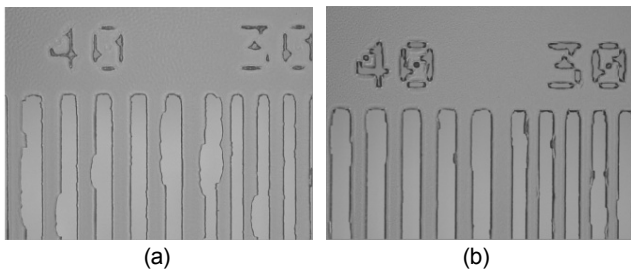
Figure 6. BM pattern properties with different UV exposure quantities and CD values: (a) CD 17.1 \mu\text{m} (80 mJ applied onto the formula 2 coated film); (b) CD 26.1 \mu\text{m} (150 mJ applied onto the formula 2 coated film).
