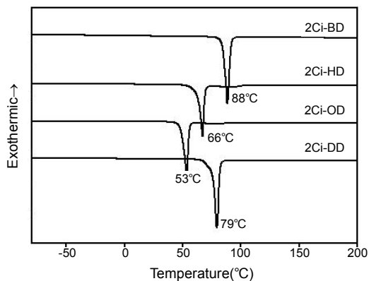
Figure 4. DSC thermograms of oligomeric cinnamates.
