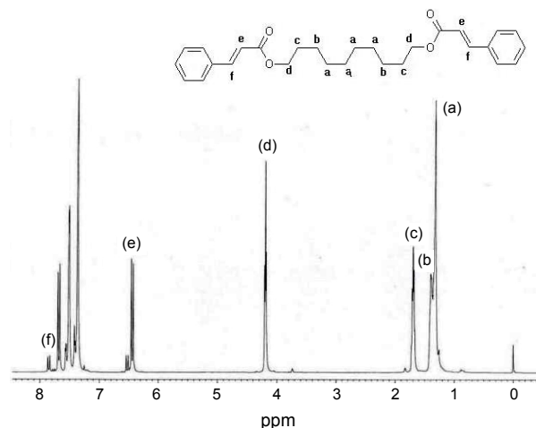
Figure 2. ^1\text{H-NMR} spectrum of 2Ci-DD.
