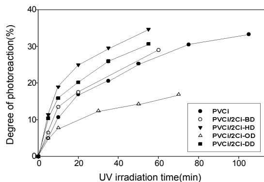
Figure 6. Degree of photoreaction with the UV irradiation time.
