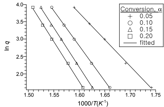
Figure 5. Flynn-Wall-Ozawa plot of TGA results for Sample1, showing that the activation energy of degradation may be obtained from the slope.
