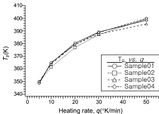
Figure 3. Peak temperature, at which maximum reaction rate occur, for the samples as a function of heating rate.
