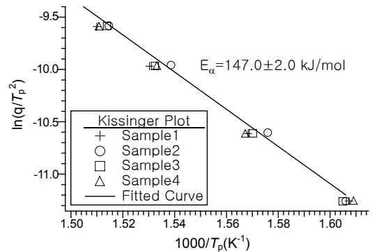
Figure 4. Kissinger plot of TGA results, showing that the activation energy of degradation may be obtained from the slope.
