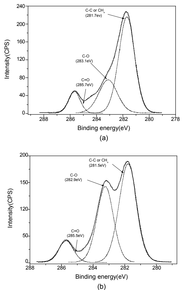
Figure 2. C1s deconvolution spectra of silicone hydrogels incorporated with PEG-MEM (MW = 300 g/mol): (a) 0 wt%; (b) 47.4 wt%.
