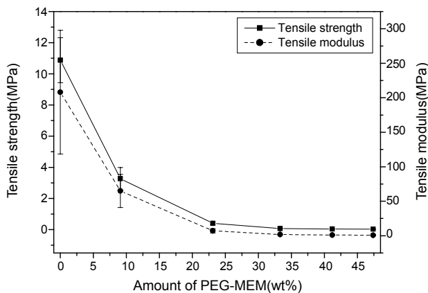
Figure 7. Tensile strength and moduli of silicone hydrogels incorporated with PEG-MEM (MW = 300 g/mol) (n = 5).
