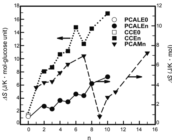
Figure 9. Plot of transition entropies ( \Delta S ) of PCALE0, 21 PCALEn, CCE0, 22 CCEn, 22 and PCAMn 9 against n : (□, ■, □, ●) at T_c ; (▼) at the smectic-to-liquid phase transition point ( T_{si} ).
