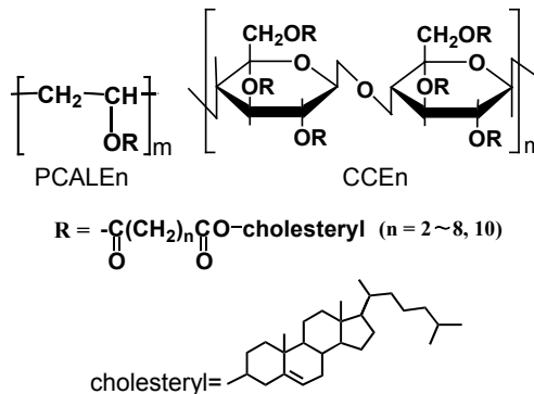
Figure 1. Chemical structures of PCALEn and CCEn.
