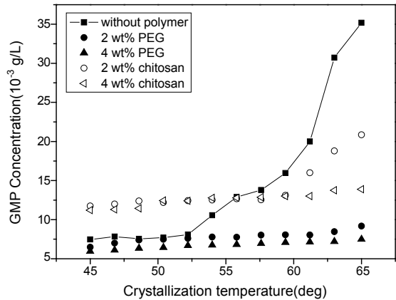
Figure 3. Effect of polymer addition on GMP solubility as a function of temperature.
