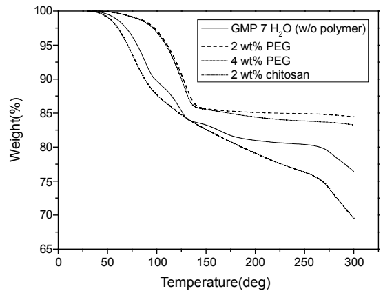
Figure 7. TGA analysis of GMP crystals formed by drowning-out crystallization at 45 °C.
