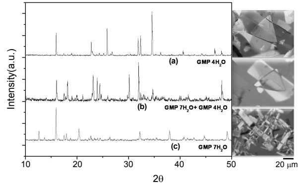
Figure 2. X-ray diffraction (XRD) and optical microscopy (OM) results of the two crystalline hydrates of GMP. GMP hydrates crystallized (a) at 65 °C; (b) 50 °C; (c) 45 °C. Crystallization temperature influenced the kind of crystal hydrates.
