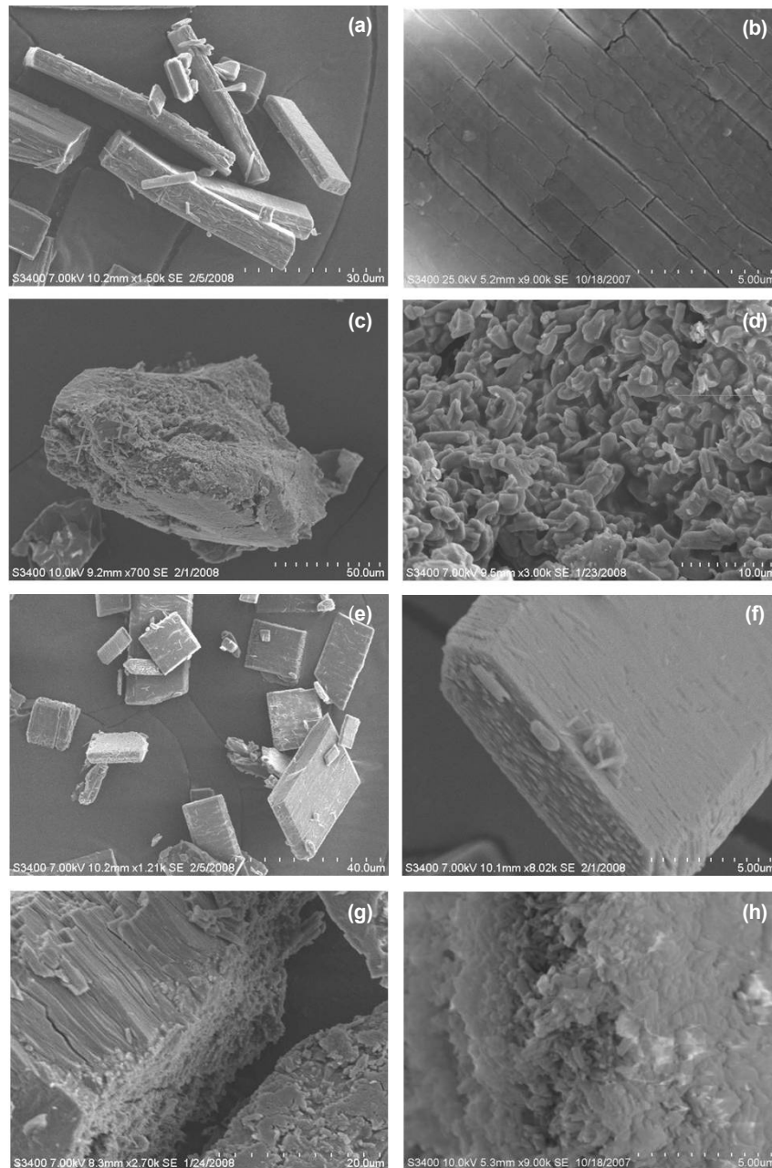
Figure 5. SEM images of GMP crystals formed by drowning-out crystallization: (a) Crystals obtained without a polymer at 45 °C; (b) crystal surface of (a); (c) crystals obtained in 2 wt% PEG solution at 45 °C; (d) crystal surface of (c); (e) crystals obtained in 2 wt% PEG solution at 25 °C; (f) crystal surface of (e); (g) in 4 wt% PEG solution at 45 °C; (h) in 2 wt% chitosan solution 45 °C.
