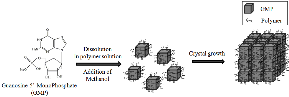
Figure 1. Schematic representation of polymer-directed dawning-out crystallization.
