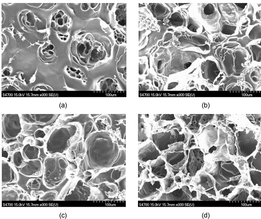
Figure 7. SEM photographs of pore in hydrogel by enzyme unit: (a) 0 unit; (b) 10 unit; (c) 20 unit; (d) 40 unit.
