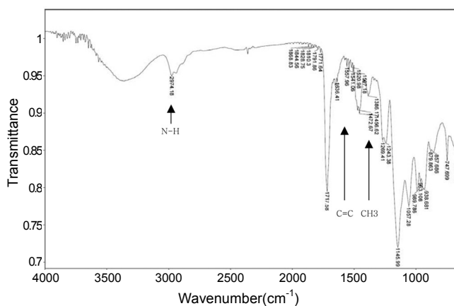
Figure 2. FT-IR spectra of hydrogel.
