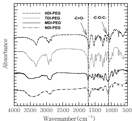
Figure 1. FT-IR spectra of the synthesized polyurethanes in this study.
