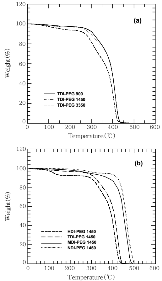
Figure 4. TGA curves of synthesized polyurethanes: (a) TDI based polyurethane with different M_w of PEG and (b) PEG 1450 with various hard segments.
