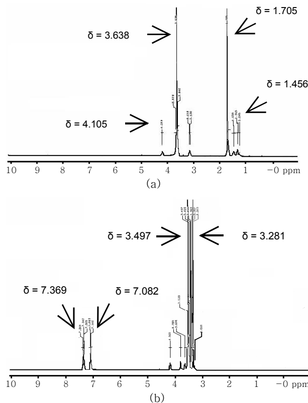
Figure 2. 1 H-NMR spectra of synthesized polyurethane: (a) HDI-PEG and (b) MDI-PEG.
