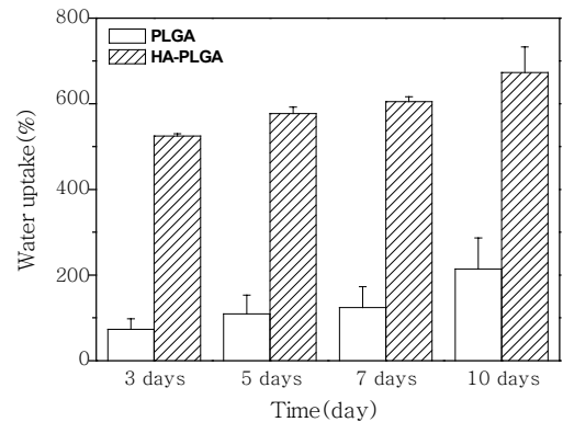
Figure 4. Water-uptake ability of PLGA and HA-PLGA scaffold by means of emulsion freeze-drying method.
