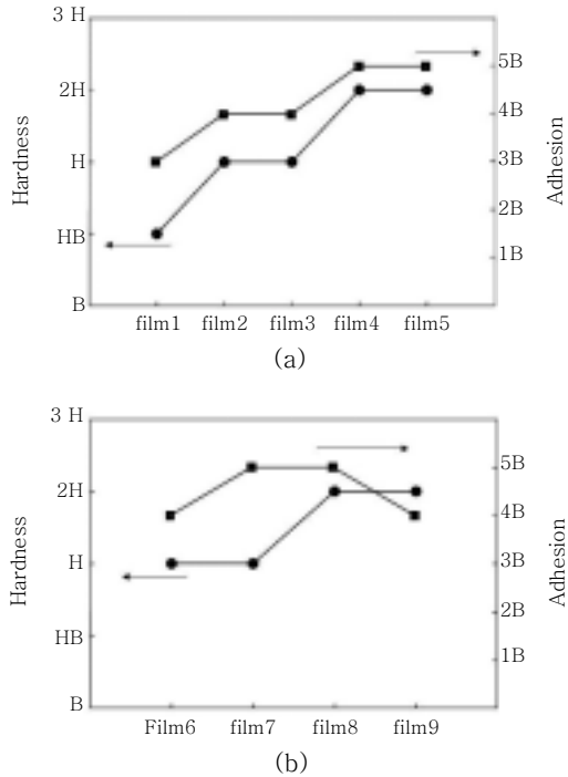
Figure 8. Hardness and adhesion results of organic-inorganic hybrid films. (a) effect by mole-ratio of ORMOSILs, and (b) effect by content ratio of ORMOSIL and acrylic resin.
