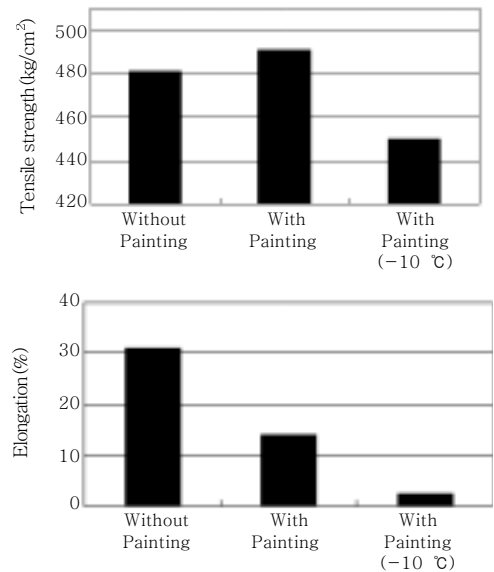
Figure 10. Toughness depends on environmental factors.
