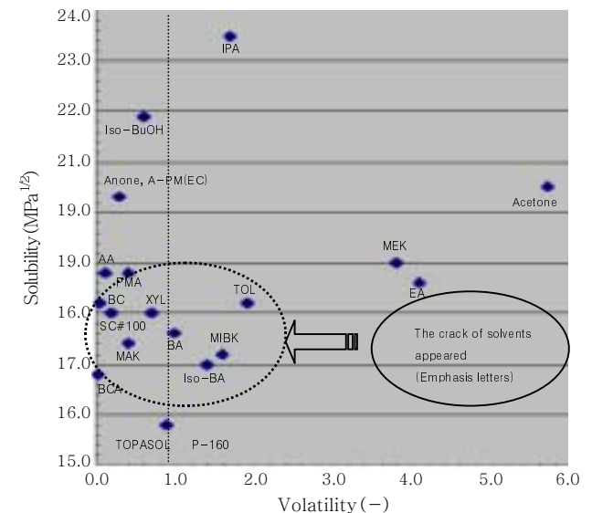
Figure 7. Volatility vs solubility with various solvents.
