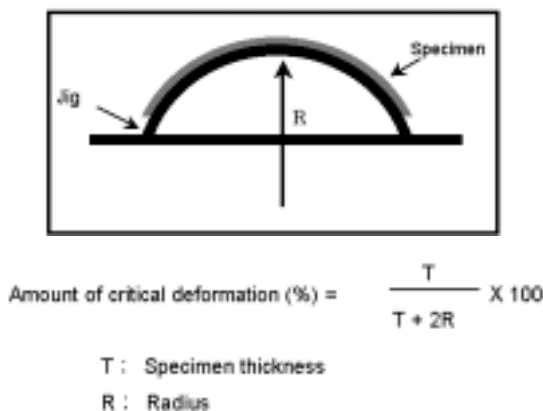
Figure 4. The test method of ESCR.
