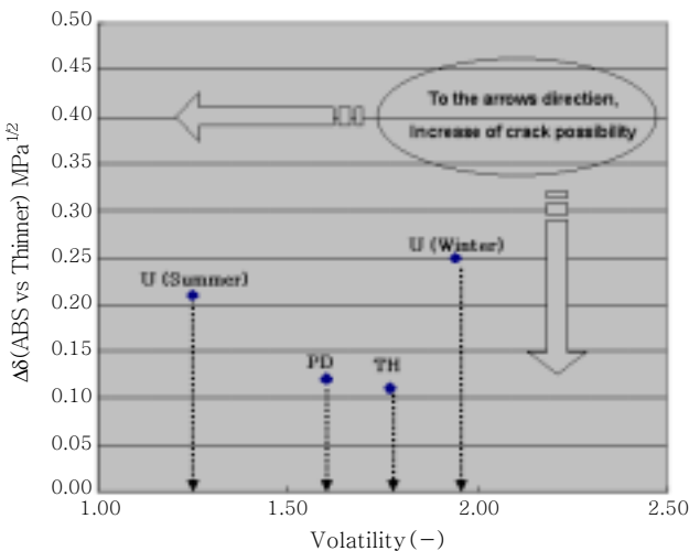
Figure 6. Volatility vs solubility with various thinners.
