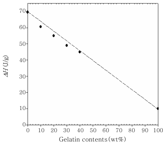
Figure 7. Total enthalpy ( \Delta H ) for PVA/GEL blend membranes as a function of GEL contents (dashed line : theoretical value ( \Delta H_t )).
