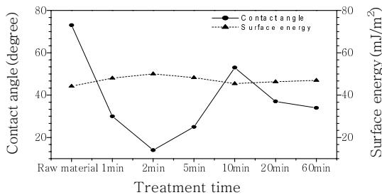
Figure 3. Change of contact angle and surface energy with plasma treatment time.
