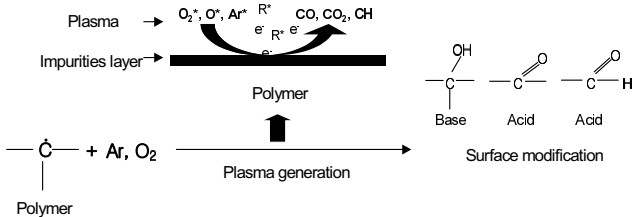
Figure 7. Mechanism for the formation of surface functional group by plasma treatment.
