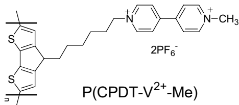
Figure 6. Structure of P(CPDT-V-Me).
