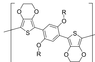
P(BEDOTPh-2V)
