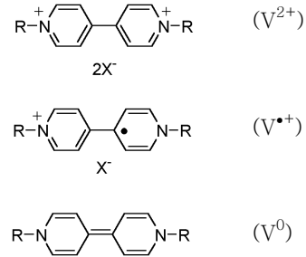
Figure 2. The oxidation states of viologen. The corresponding symbols are shown in the parenthesis.
