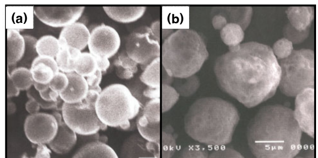
Figure 2. Scanning electron micrographs of microsphere. (a) immediately after preparation and (b) 41 days after pDNA release.
