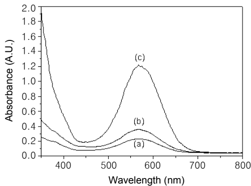
Figure 3. UV/vis spectra of (a) CA-COSP1, (b) CA-COSP2, and (c) CA-COSP3 films normalized by thickness ( \sim 6 \mu\text{m} ) after irradiation of UV for 240 sec, respectively.
