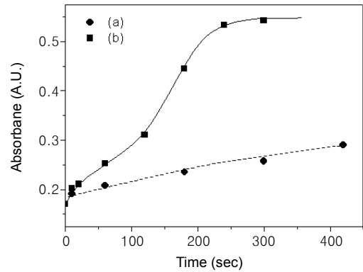
Figure 8. Change of absorbance at 580 nm for CA-COSP3 film with irradiation of (a) 254 nm and (b) 365 nm UV light.
