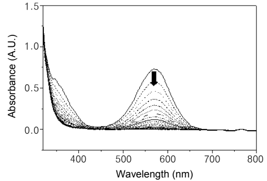
Figure 4. Change of absorption spectra for CA-COSP3 in DMSO upon 365 nm irradiation; [\text{CA-COSP3}] = 0.093 .
