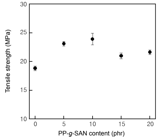
Figure 1. Tensile strength of the PP/ABS (54/46 wt%) blend containing PP-g-SAN compatibilizer.
