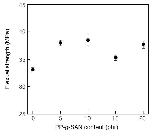
Figure 2. Flexural strength of the PP/ABS (54/46 wt%) blend containing PP-g-SAN compatibilizer.
