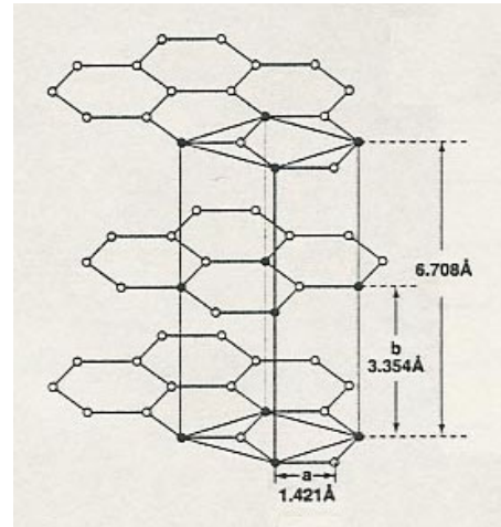
Figure 1. Crystal structure of the expandable graphite.
