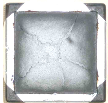
Figure 18. Char formation of the NBR/GTR compounds (specimen 6).
