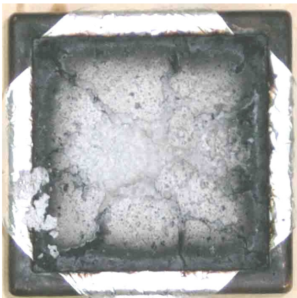
Figure 15. Char formation of the NBR/GTR compounds (specimen 1).
