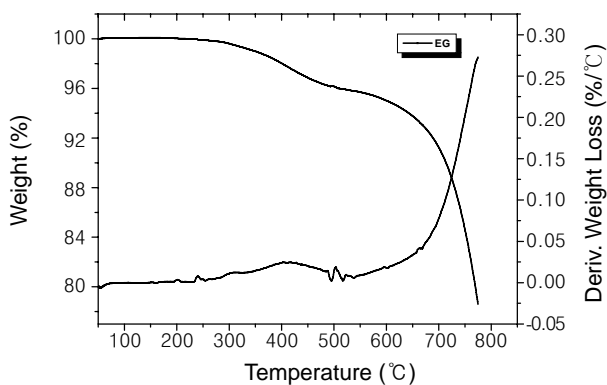
Figure 3. TGA/DTG curves of expandable graphite (in air).
