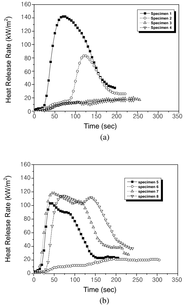
Figure 10. Heat release rate of the NBR/GTR compounds (specimen 1~8).
