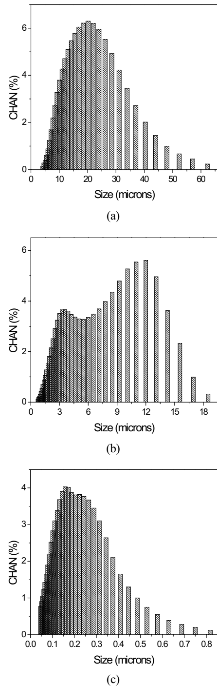
Figure 3. Influence of the polymerization methods on the average particle size and particle size distribution of PVAc nanoparticles;(a) EM, (b) EM-2, and (c) M-EM.
