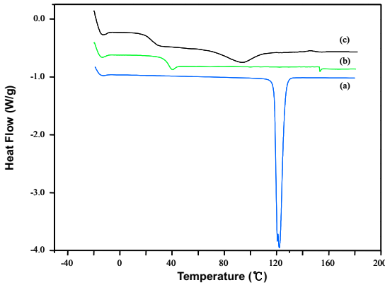
Figure 6. DSC thermograms of (a) IP, (b) PLGA, and (c) IP 10% loaded PLGA MSs.
