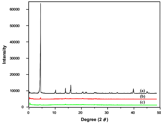
Figure 5. XRD of (a) IP, (b) PLGA, and (c) IP 10% loaded PLGA MSs.
