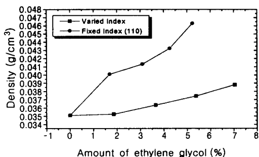
Figure 7. Effects of ethylene glycol contents on density.
