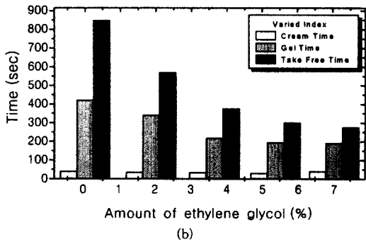
Figure 1. Effects of ethylene glycol contents on reactivity. (a) when isocyanate index is fixed and (b) when isocyanate index is varied.
