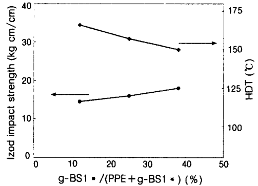
Figure 3. Changes in Izod impact strength and heat deflection temperature as a function of g-BS1* content in PPE phase.
