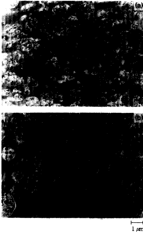
Figure 10. Transmission electron micrographs of PA/PPE/SEBS blends for two g-BS*'s with different rubber particle sizes: (a) 0.1 μm and (b) 0.3 μm.
