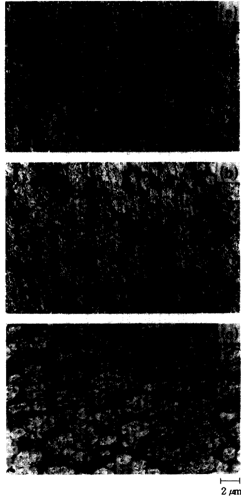
Figure 6. Transmission electron micrographs of PA/PPE/SEBS blends for various g-BS*’s having different molecular weights of grafted PS: (a) 200000, (b) 300000, and (c) 500000.
