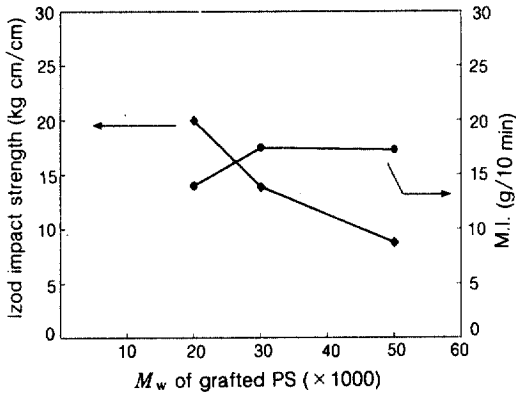
Figure 5. Changes in Izod impact strength and melt flow index as a function of molecular weight of grafted PS.
