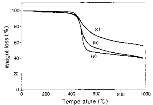
Figure 2. TGA curves of (a) P(OT/FPT)(2:1), (b) P(OT/FPT)(1:1), and (c) P(OT/FPT)(1:2).
