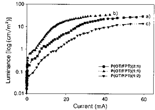
Figure 10. I-L curves of (a) P(OT/FPT)(2:1), (b) P(OT/FPT)(1:1), and (c) P(OT/FPT)(1:2).
