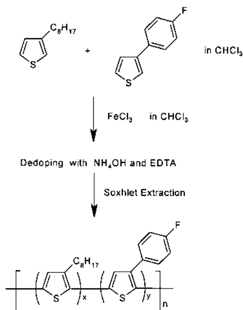
Figure 1. Synthetics of poly[3-octylthiophene-co-3-(4-fluorophenyl)thiophene] (x:y=2:1, 1:1, 1:2).
