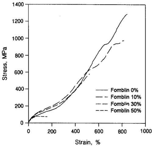
Figure 2. Stress-strain curves of PTMG-series polyurethanes.
