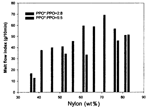
Figure 8. Variation of melt flow index as a function of nylon amount in the final ternary blend.
