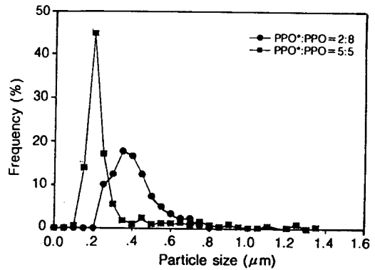
Figure 5. Domain size distribution of ternary blends containing 52 wt% nylon and PPO with PPO*:PPO=2:8 and 5:5.
